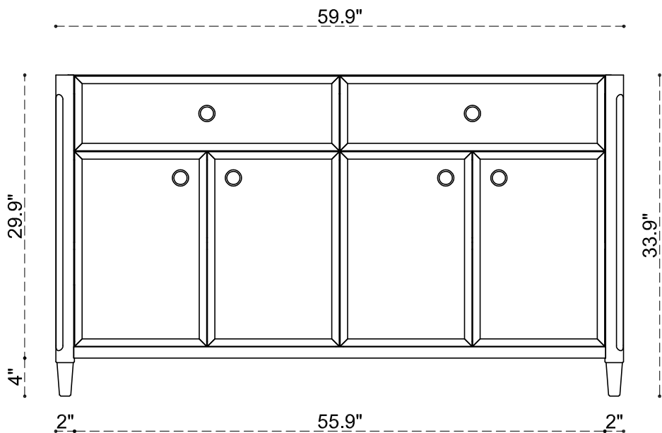
FRONT VIEW
