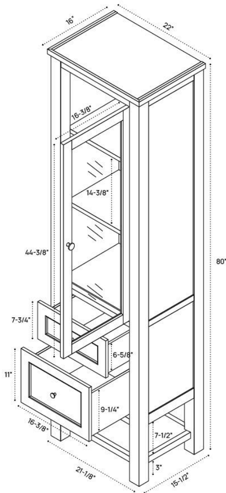
SIDE VIEW
