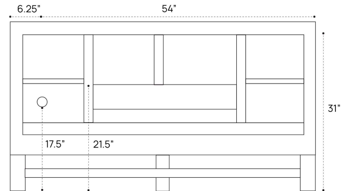
BACK VIEW
