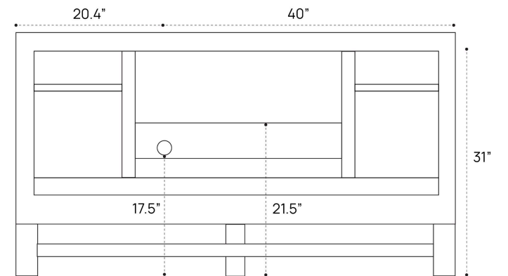
BACK VIEW
